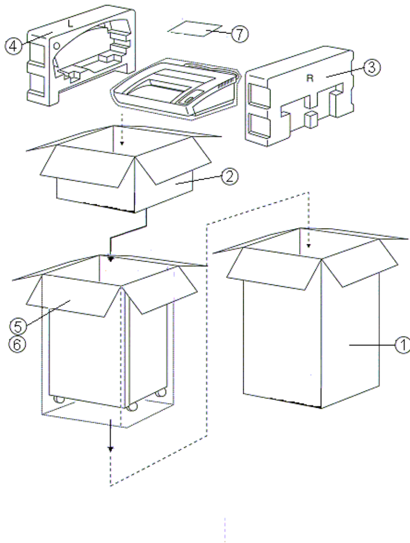
Section 8.0 5220S/5230S/5260X. Parts List 5220S/5230S/5260X. Packaging Exploded View Figure 8. 8
