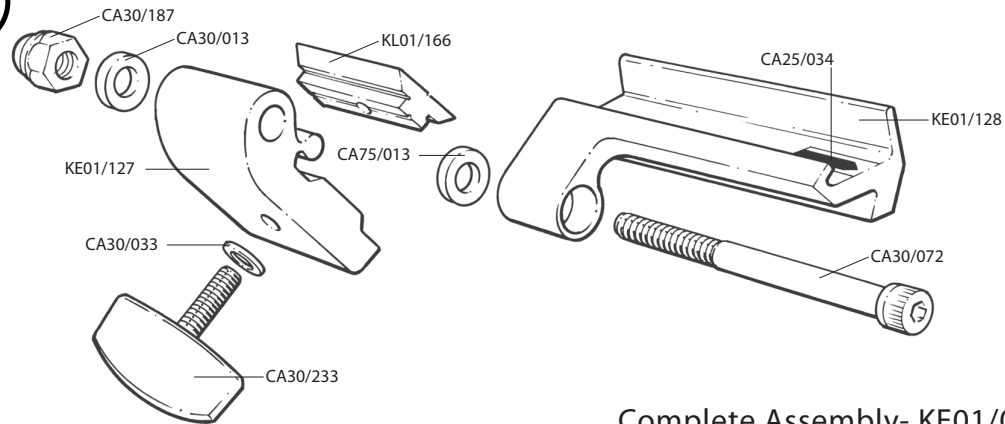
Complete Assembly- KE01/010
