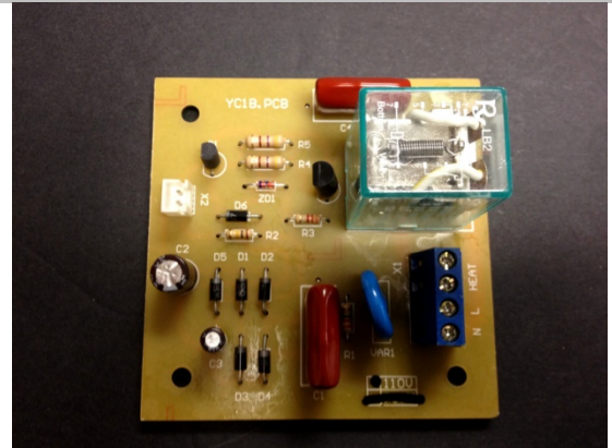
#37 – PCB-YCL-600HL
