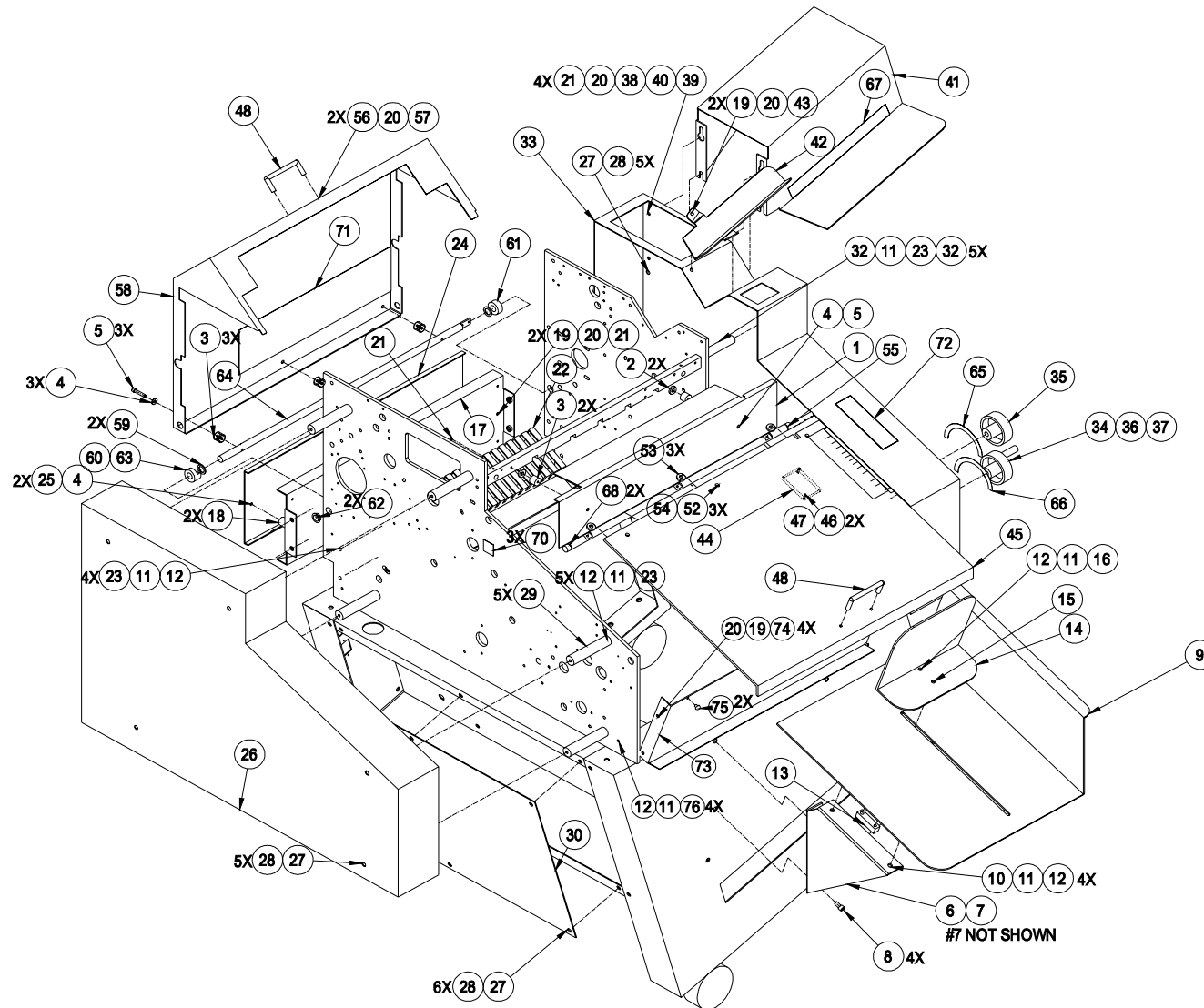
FIGURE 8.1 COVERS
