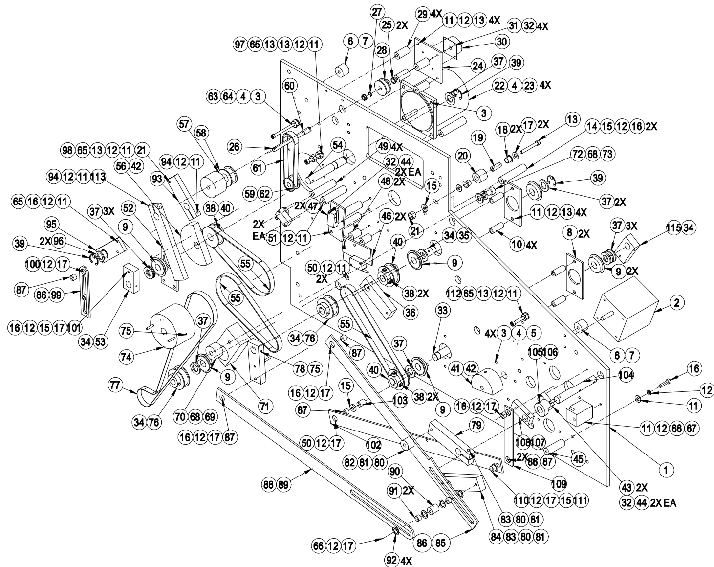
FIGURE 8.7 REAR ASSEMBLY
