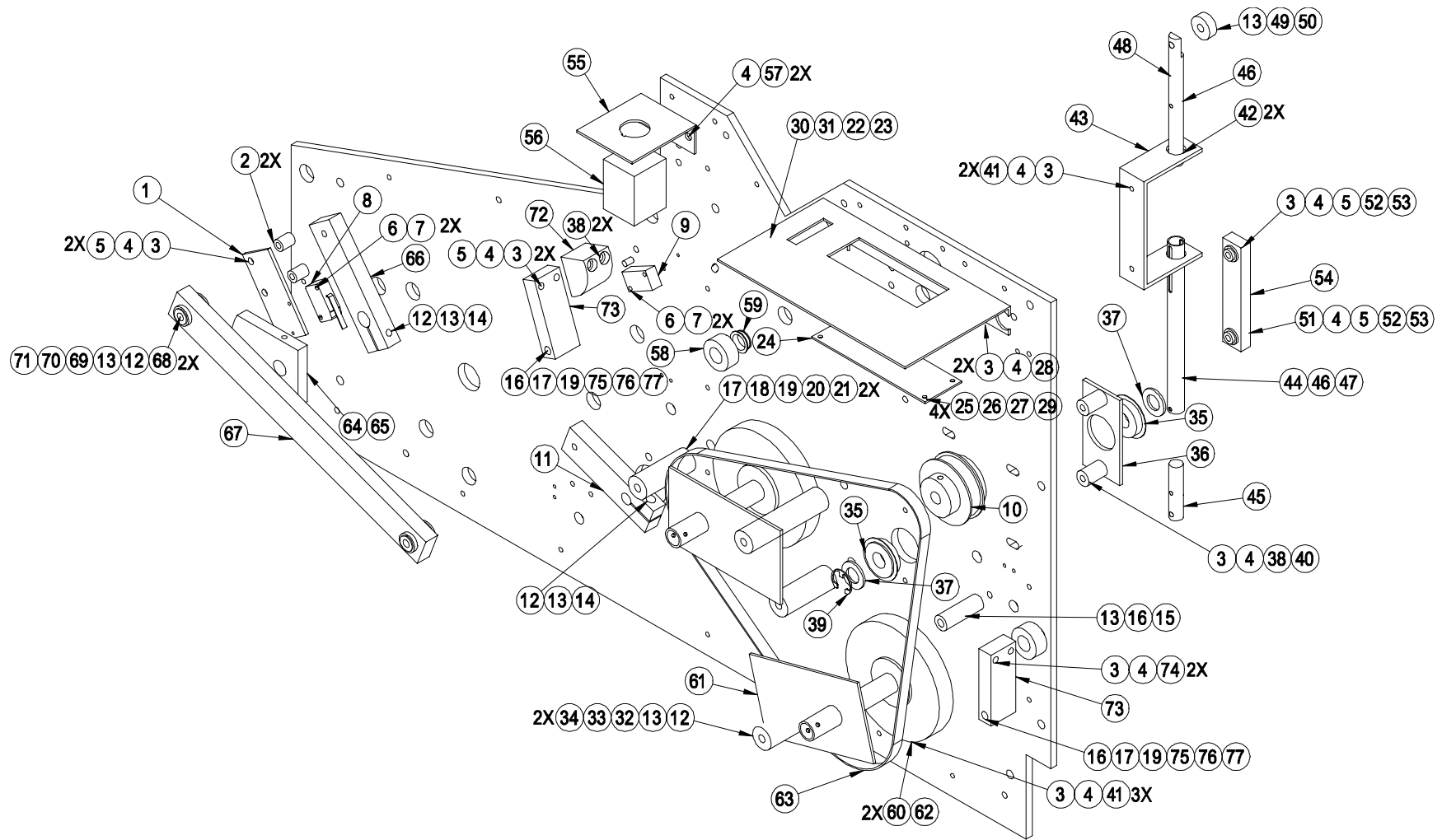
FIGURE 8.5 FRONT PANEL ASSEMBLY
