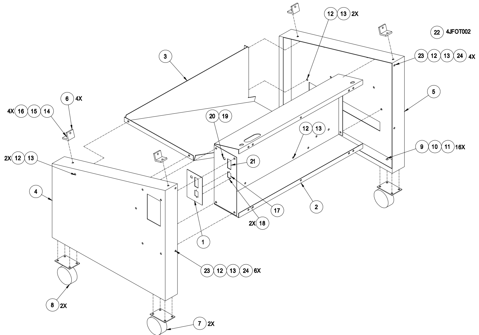
FIGURE 8.2 BASE ASSEMBLY
