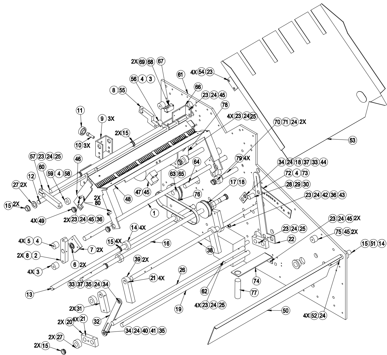
FIGURE 8.6 CENTER ASSEMBLY
