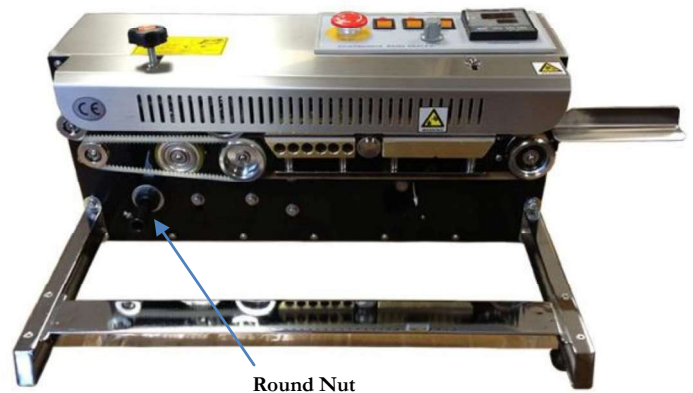
Figure 18. After removing the conveyor, remove the drive shaft and loosen the round nut.
