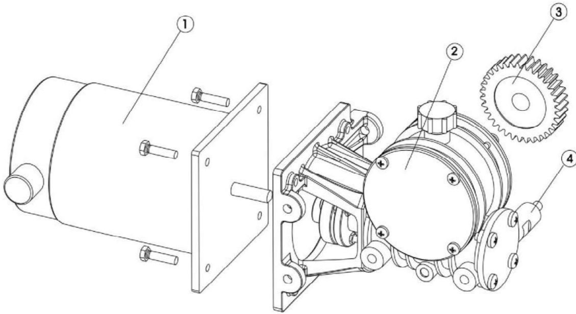
Figure 42. Motor / Turbocase
