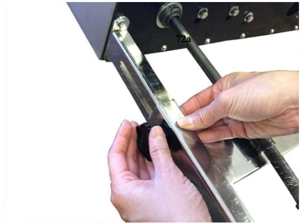
Figure 28. Tighten both sides with screw and knob. You can make adjustments to the height of your band sealer.
