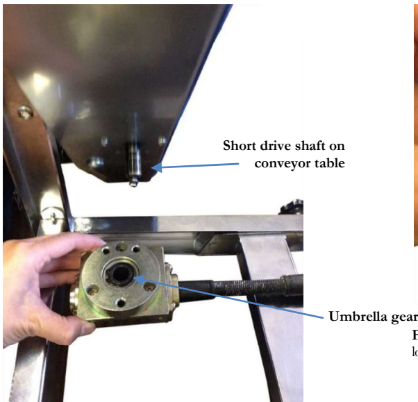
Figure 29. Insert the short drive shaft on the conveyor unto the groove of the umbrella gear.
