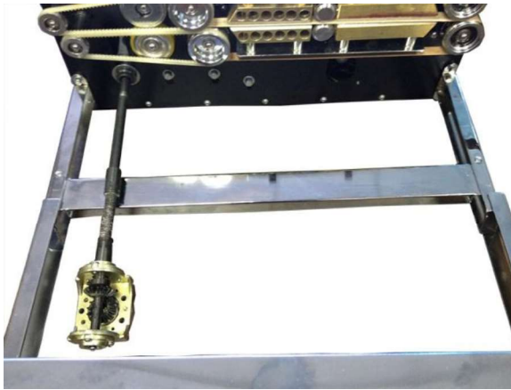
Figure 27. Insert the vertical stand on the conveyor support..
