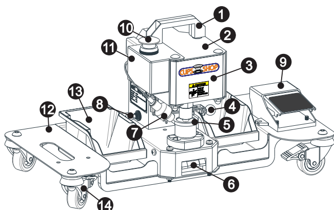
CS-TIDY-41 FB with optional Mobile Stand Accessory (CS-TIDY- W)
