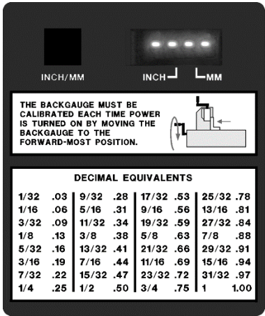
Figure 7 – Display at power up
