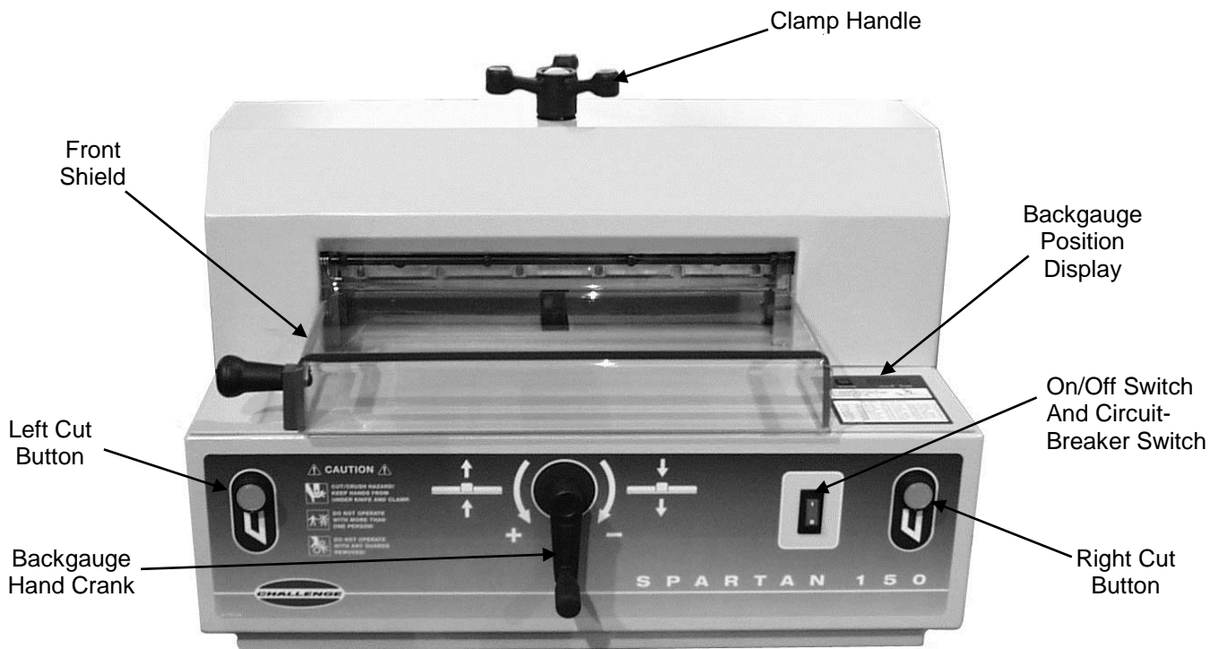
Figure 5 – Machine Controls
