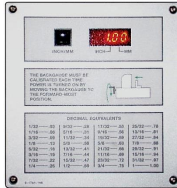
Figure 8 – Display with backgauge at 1.00 inches
