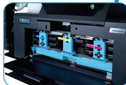
High-capacity ink tanks are easy to swap out with minimal disruption using the front access door
