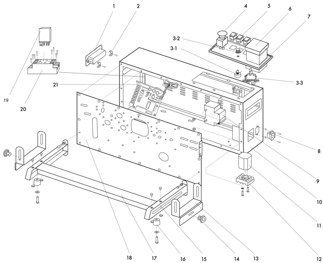
Figure 10. Sealer Body
