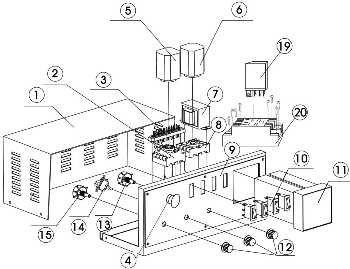
Figure 1. Controller Box
