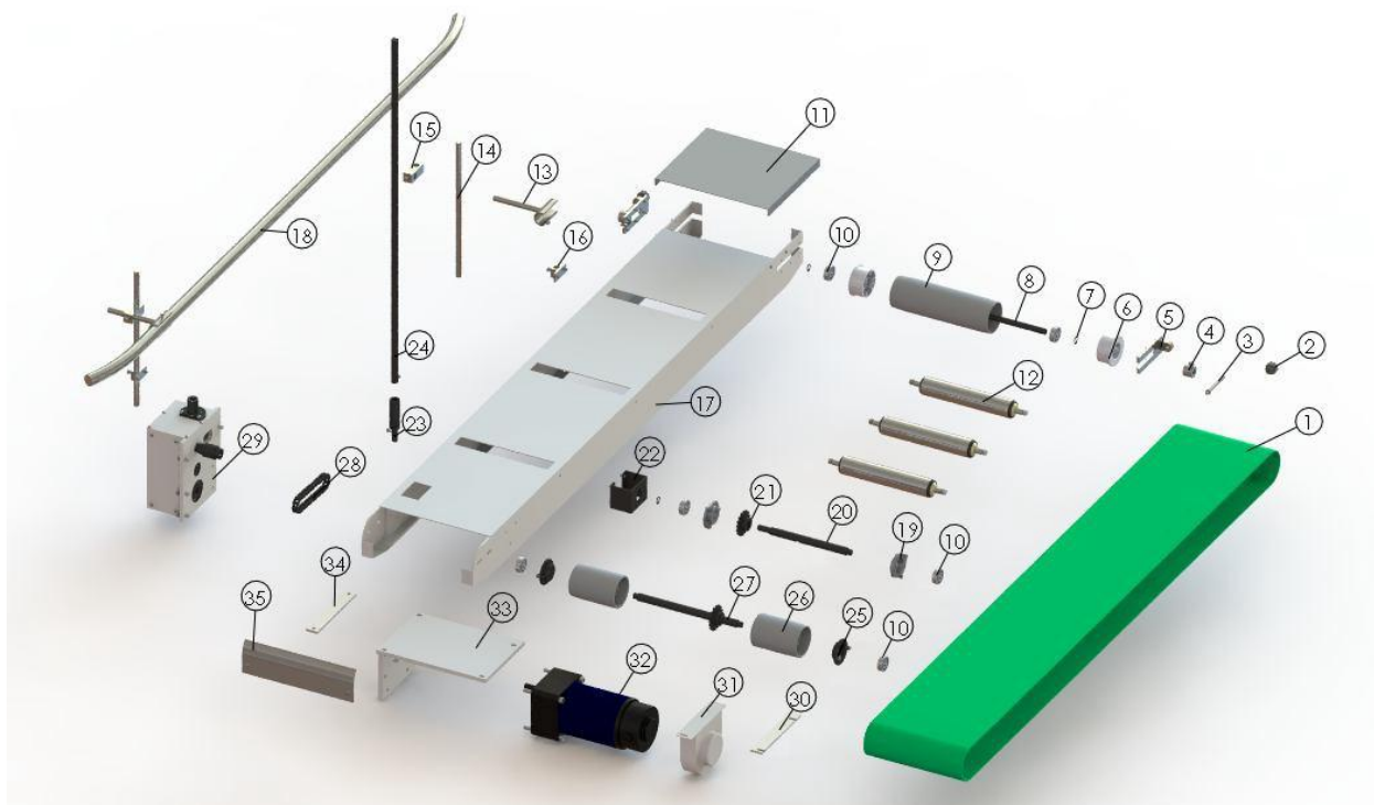
Figure 12. Conveyor Table
