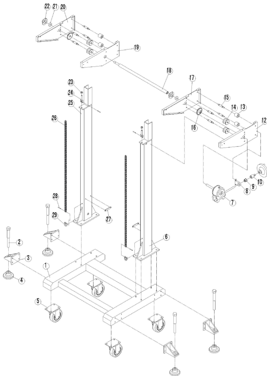
Figure 14. Sealer Rack
