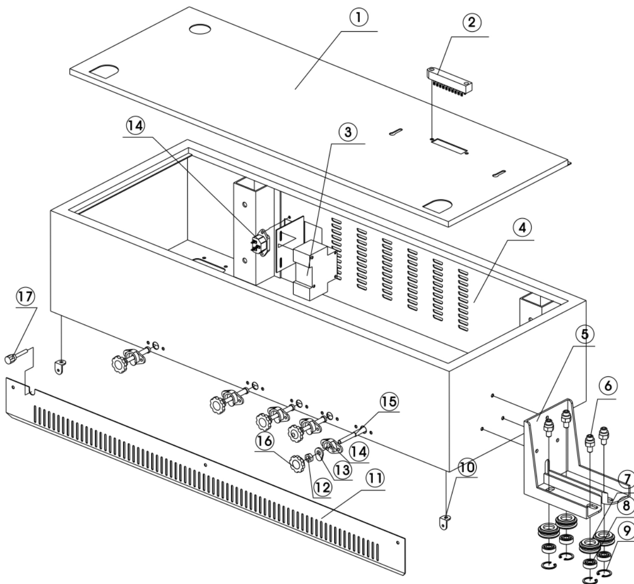
Figure 3. Sealer Body
