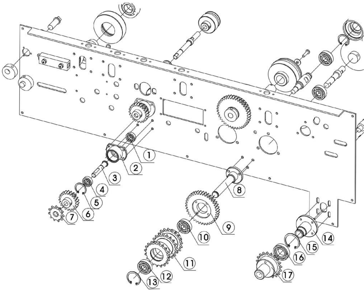
Figure 8. Sealer Body Back
