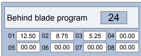
Figure 23. Value Highlighted
