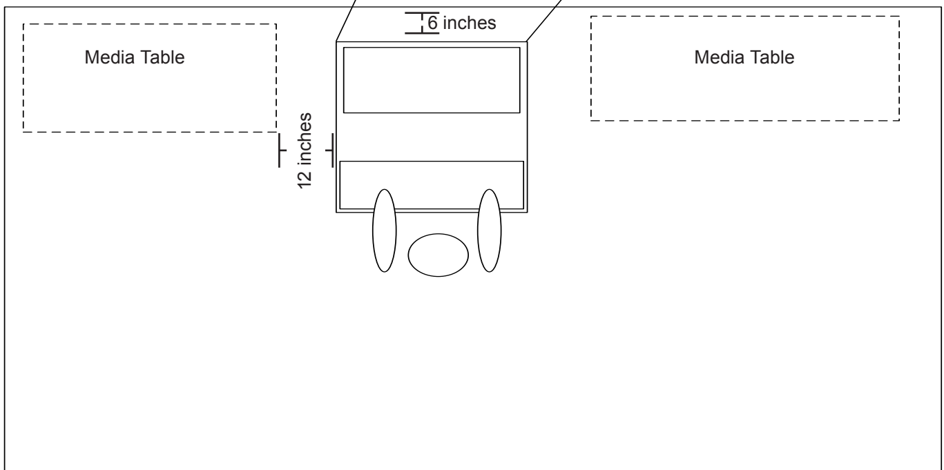
Figure 2. ProCut 20P Location
