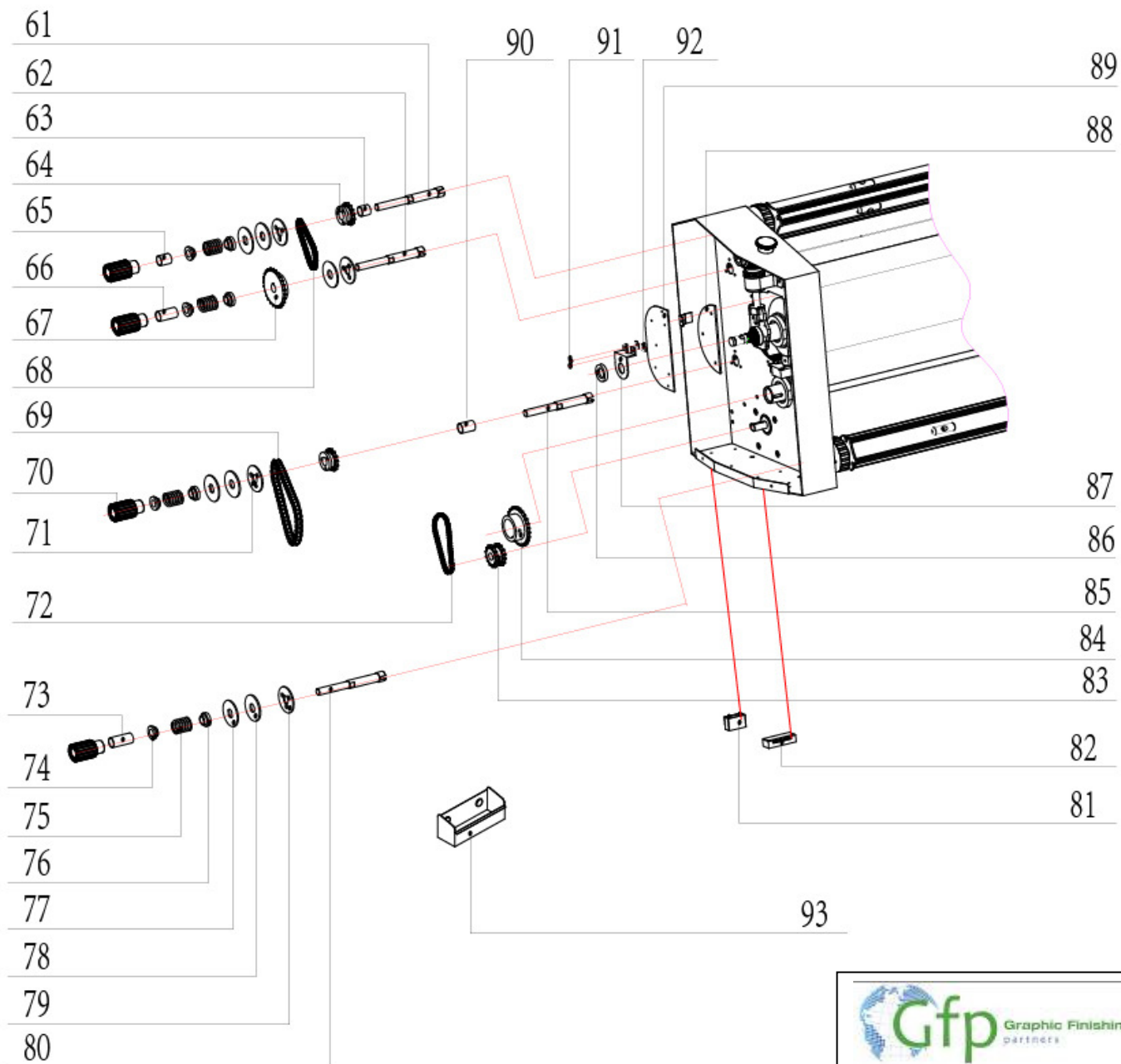
View 4 – Left side frame
