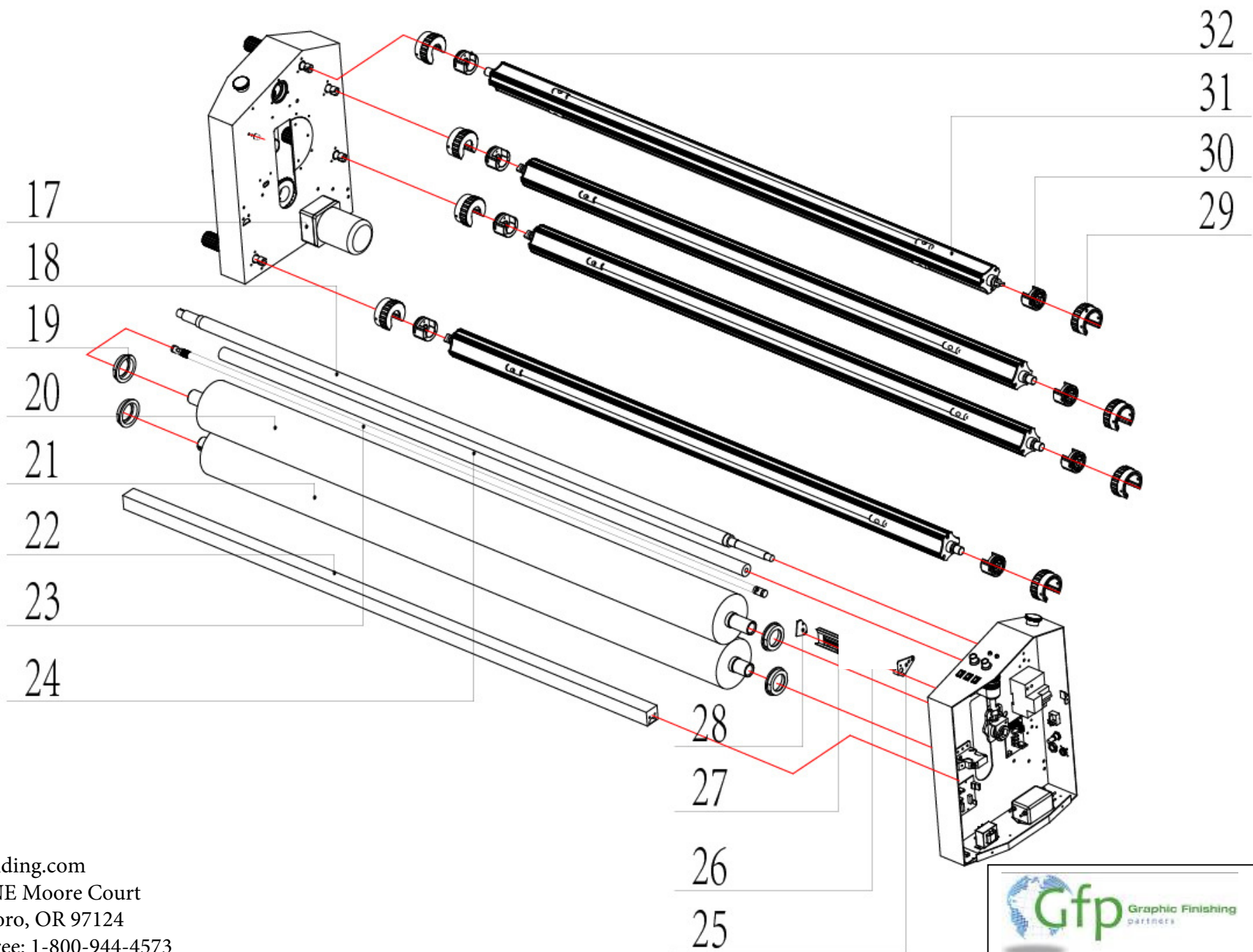
View 2 – Rollers and Shafts
