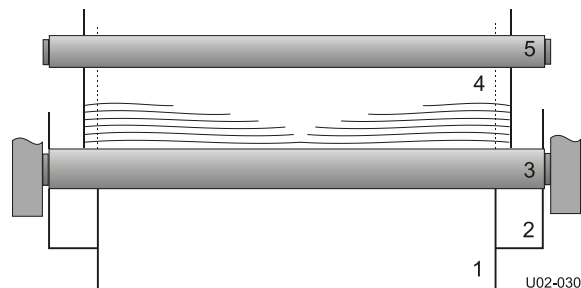
Figure 6: Wrinkles due to low pull tension
