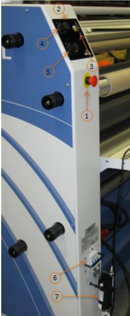
Figure 10: Rear Controls
