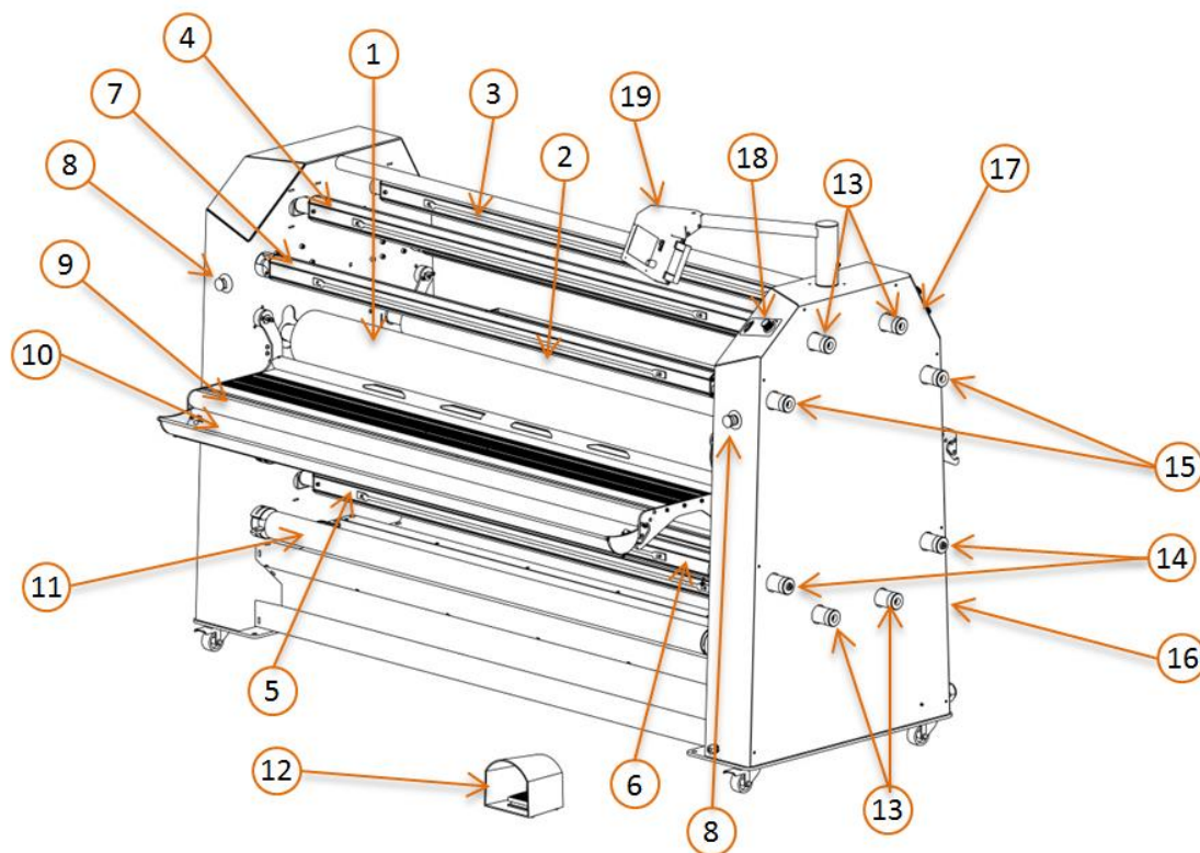
Figure 5: Parts Identification.
