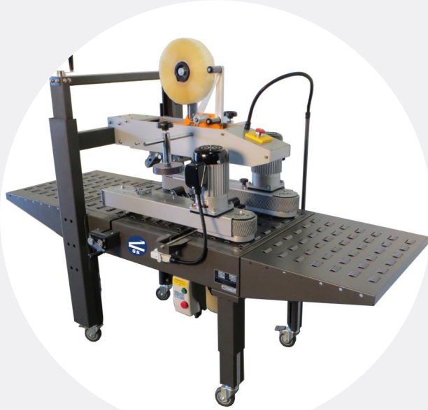
*Shown with optional infeed and discharge roller conveyors and casters
