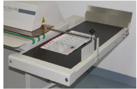
Optional 20" wide conveyor with a capacity of up to 100 books bound in 1/4 "
