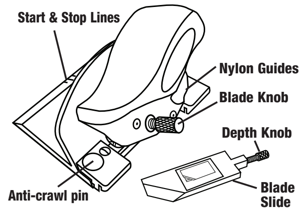
Fig. 1 #271 SINGLE BEVEL 8-PLY BLADE
