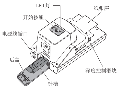
[主机后部]
