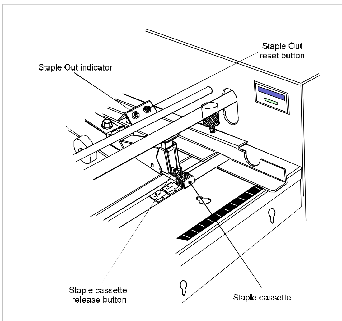
Figure 3 - Staple refill
