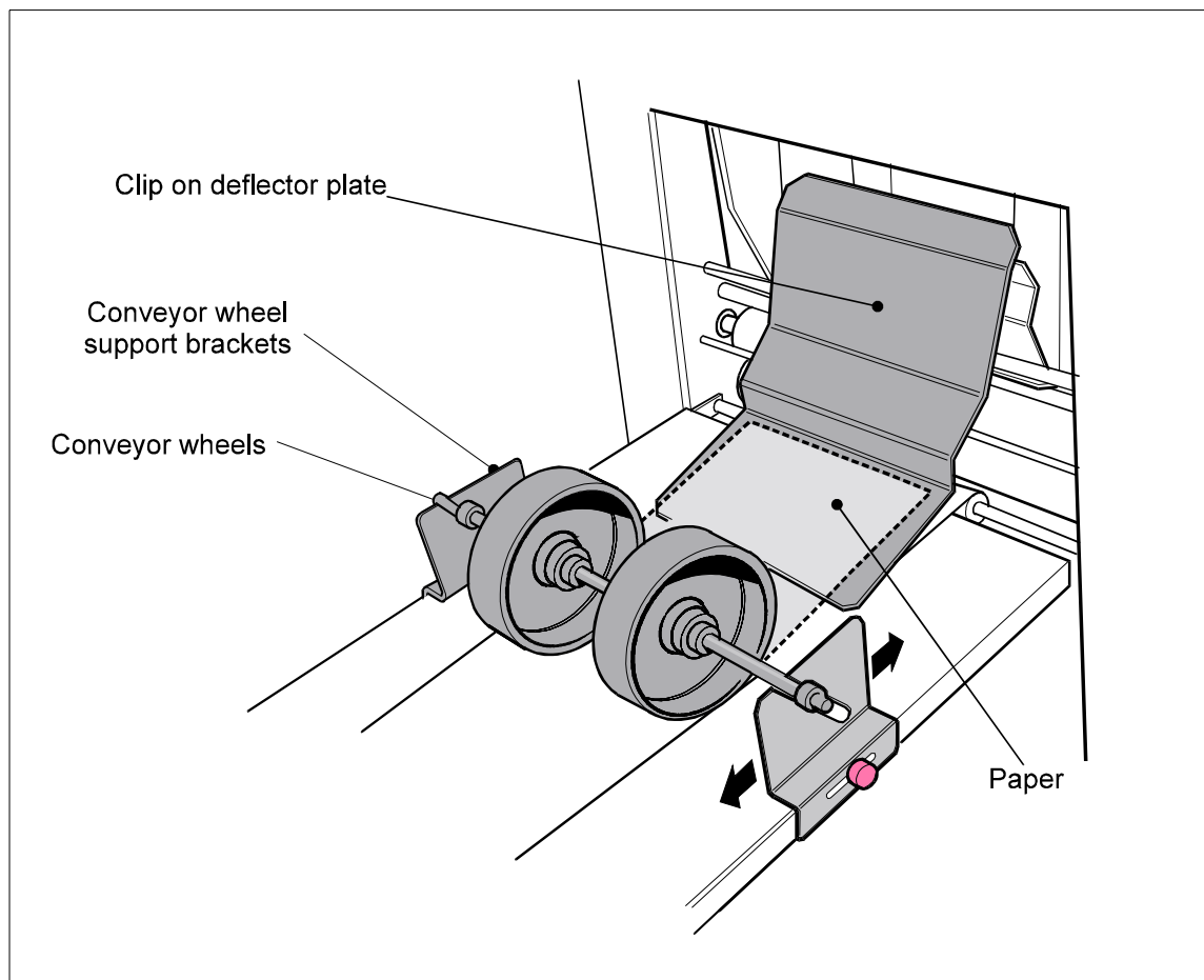
Figure 12 - Conveyor setup 2.
