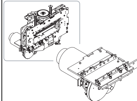
Fig.3 Reducer(1) / 減速機(1)
