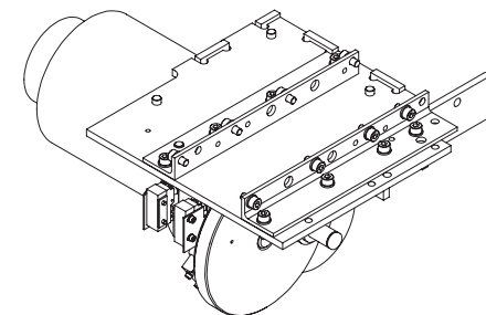
Fig.4 Reducer(2) / 減速機(2)
